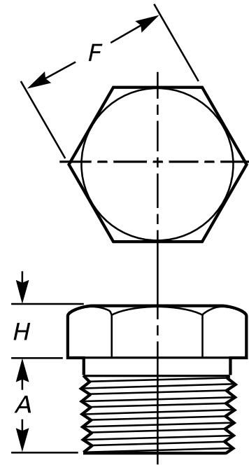
Units: Millimeters (mm)
